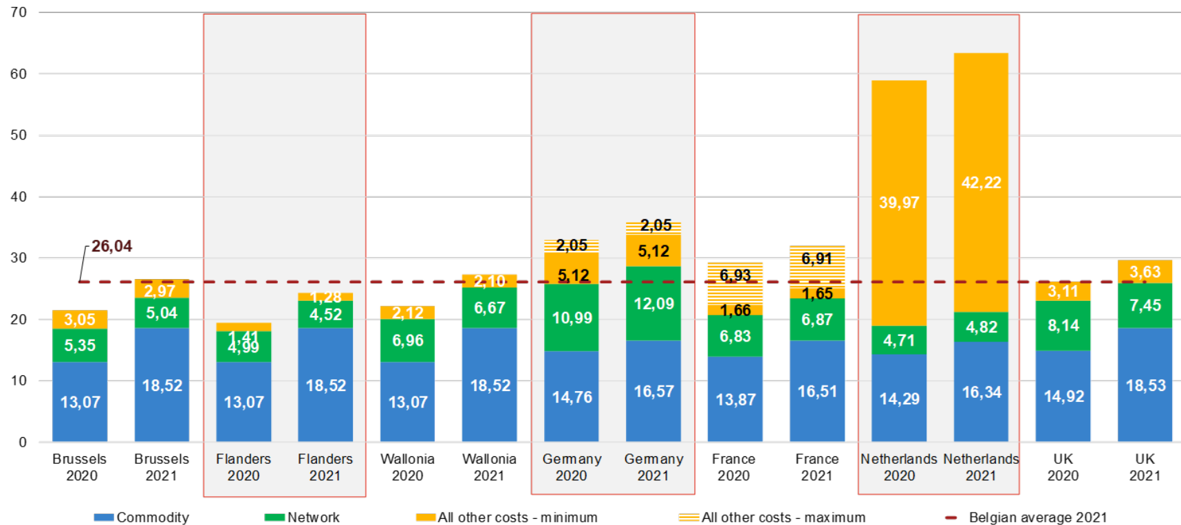
Natural gas price by component in EUR/MWh (profile G0)
