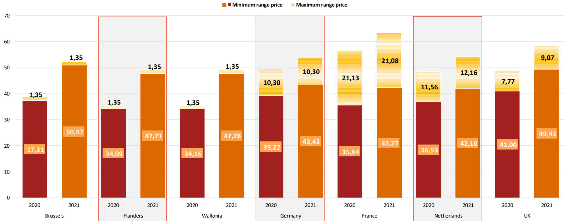
Figure 85 : Total yearly invoice in MEUR/year for industrial consumers (profile G2)
